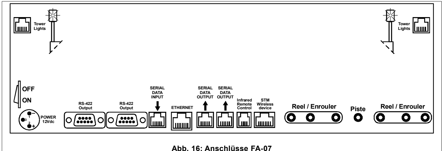
Abb. 16: Anschlüsse FA-07
